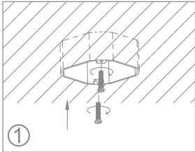
Machine screws are driven into junction box's tapped holes.
