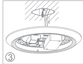
Power cord comes into the fixture.
